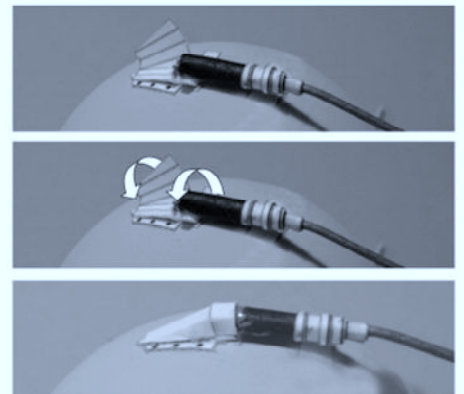
While keeping the antenna in position wrap and glue part J around it. Allow to dry.
